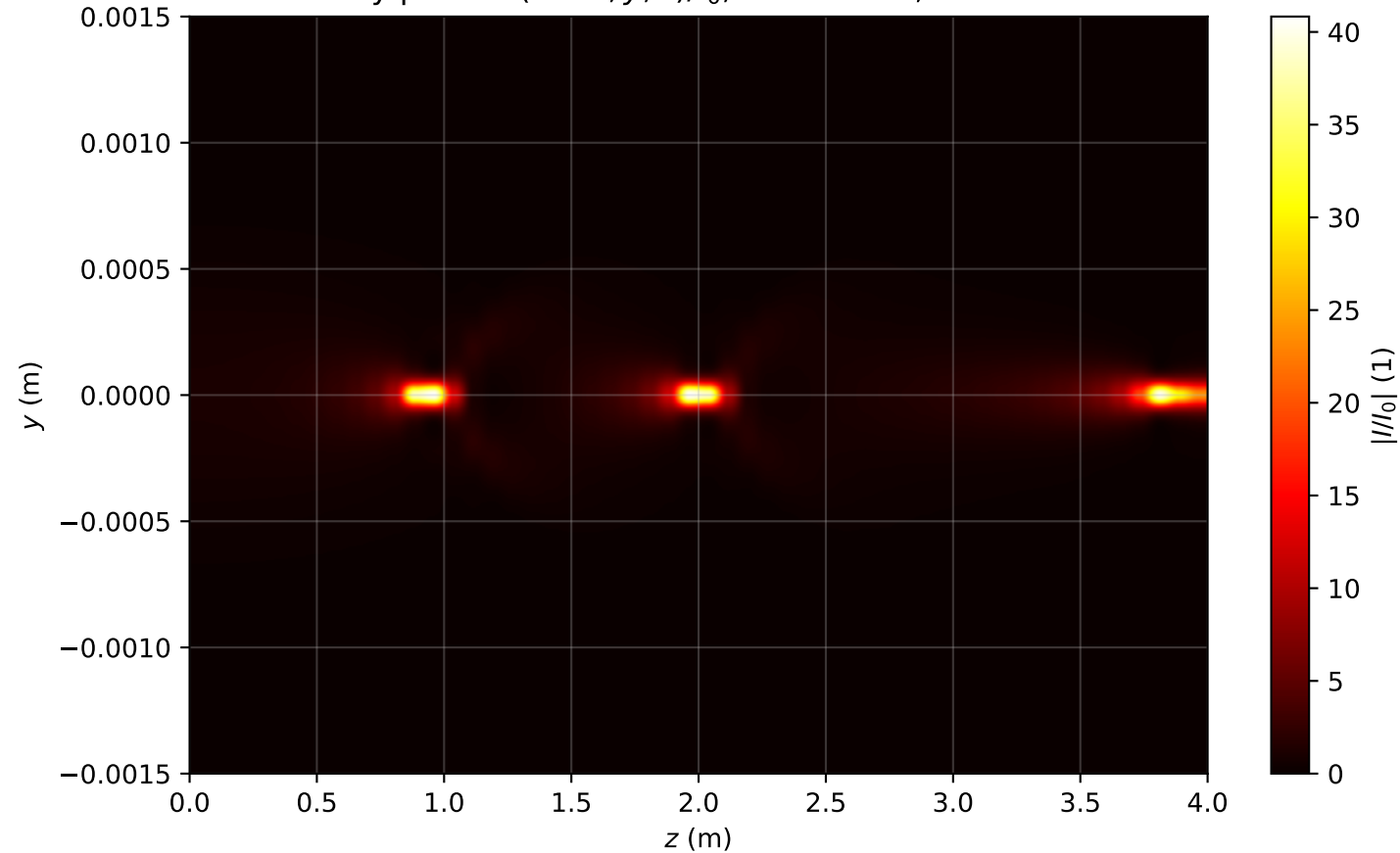
Intensity profile I(x=0, y, z)/I_0 , P_{in}=2.5P_{cr} , artificial time
